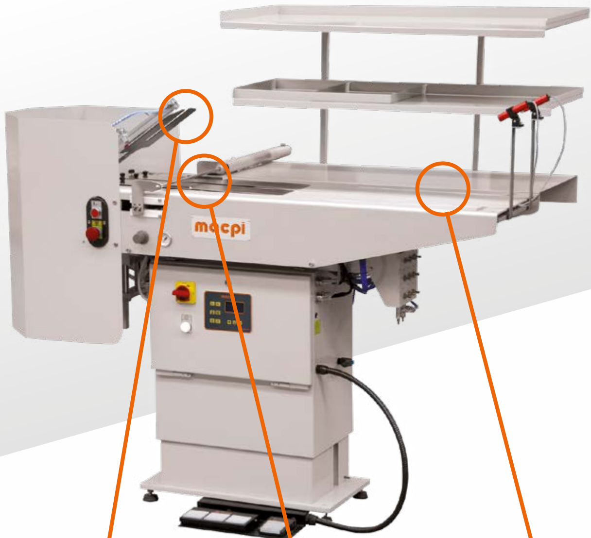
Insert System
